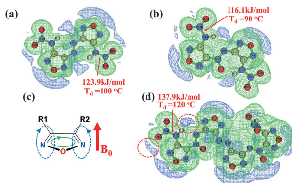
Figure 1. Visualization of the spatial magnetic properties of DNAF, DNAXF, and 1 as ICSS maps (0.70 ppm shielding, other values' shielding can be viewed in the Supporting Information). a) The ICSS map of DNAF. b) The ICSS map of DNAXF. c) The diagrammatic illustration of the relationship between external magnetic field (red arrow), induced current (green ring), and induced magnetic field (blue ring) in substituted furazan system d) The ICSS map of compound 1 .
